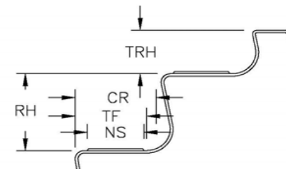
TREAD CROSS-SECTION
