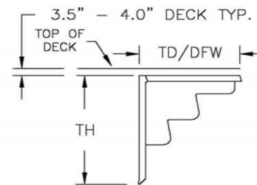
6' 3T CANT. CORNER STAIR
