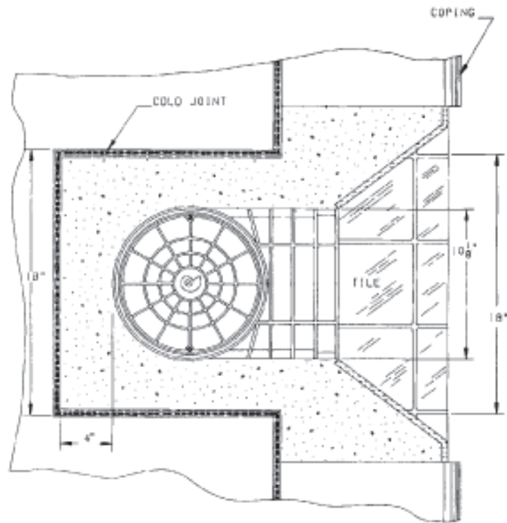
Figure 1: Top View
