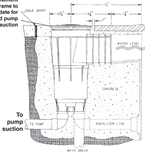
Figure 2: Section View
