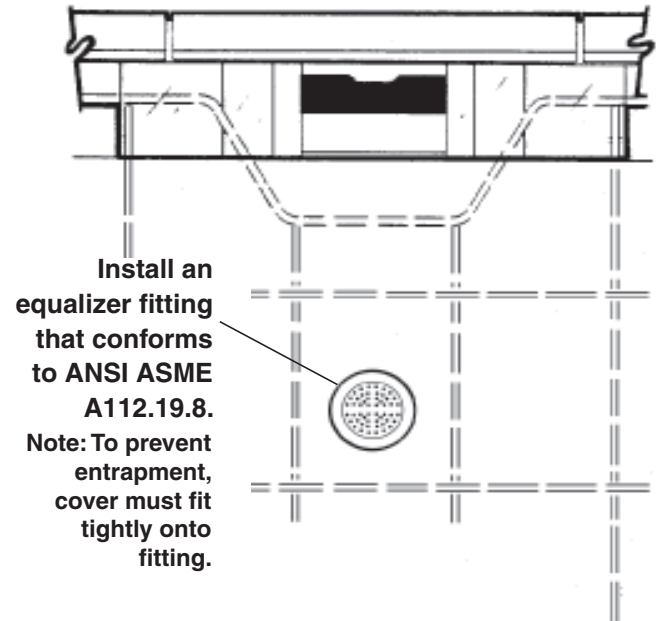
Figure 3: Front View
