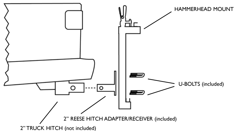
MOUNT ASSEMBLY DETAIL
