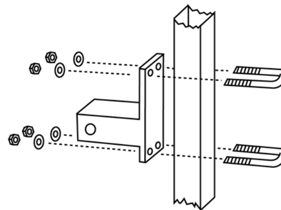
MOUNT ASSEMBLY DETAIL
