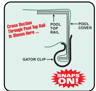
Installation Diagram
