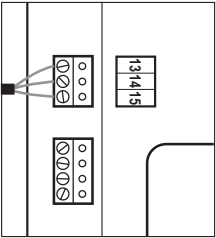
Figure 1. Remote Pool-Off Spa Connection (3-Wire Connection)
