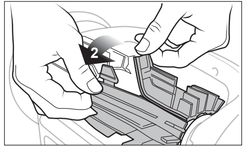
Figure 21. Undo the Tabs of the Brush
