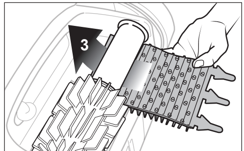
Figure 22. Install the New Brush
