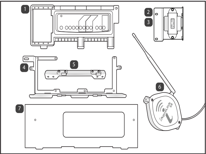
Figure 1. Kit Contents
