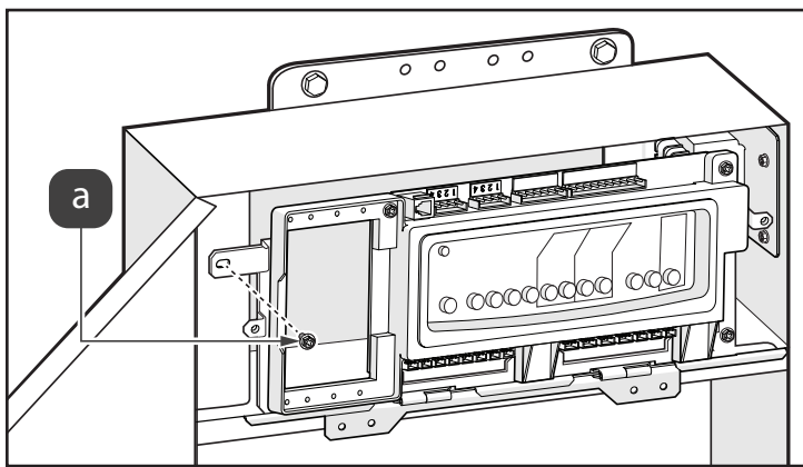
Figure 16 AquaLink RS Conversion Kit Mounting
