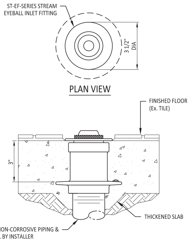
FINISHED FLOOR: ELEVATION VIEW
