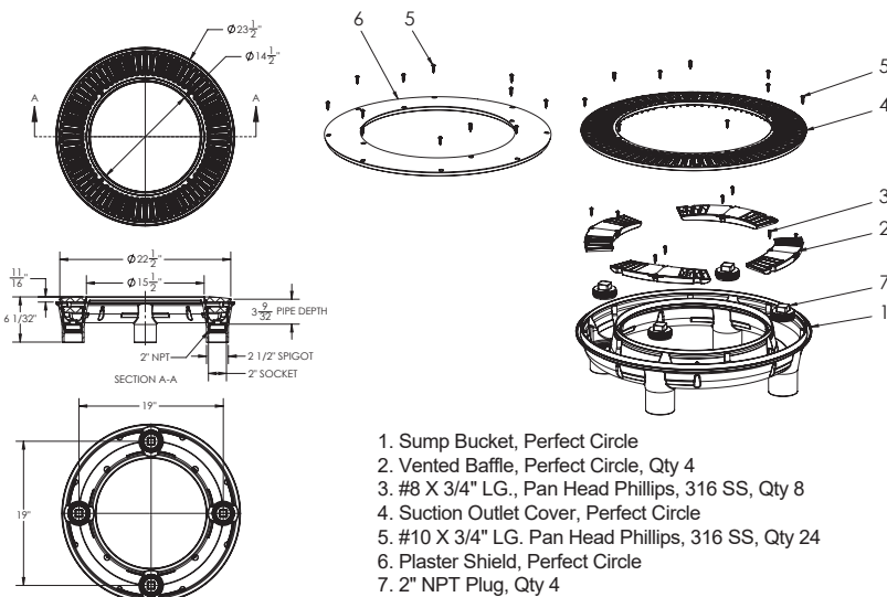
Unique water stop protects against leaks
