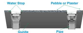
Unique water stop protects against leaks
