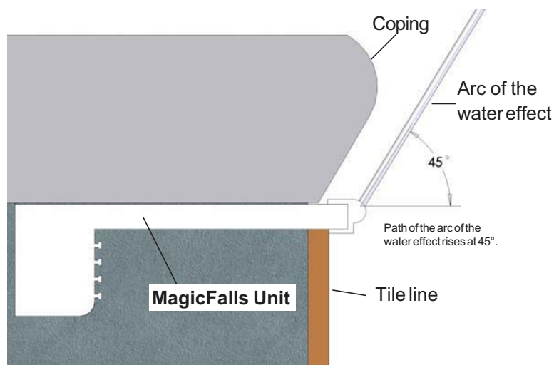
Arc of the Water Effect Must Clear Coping
