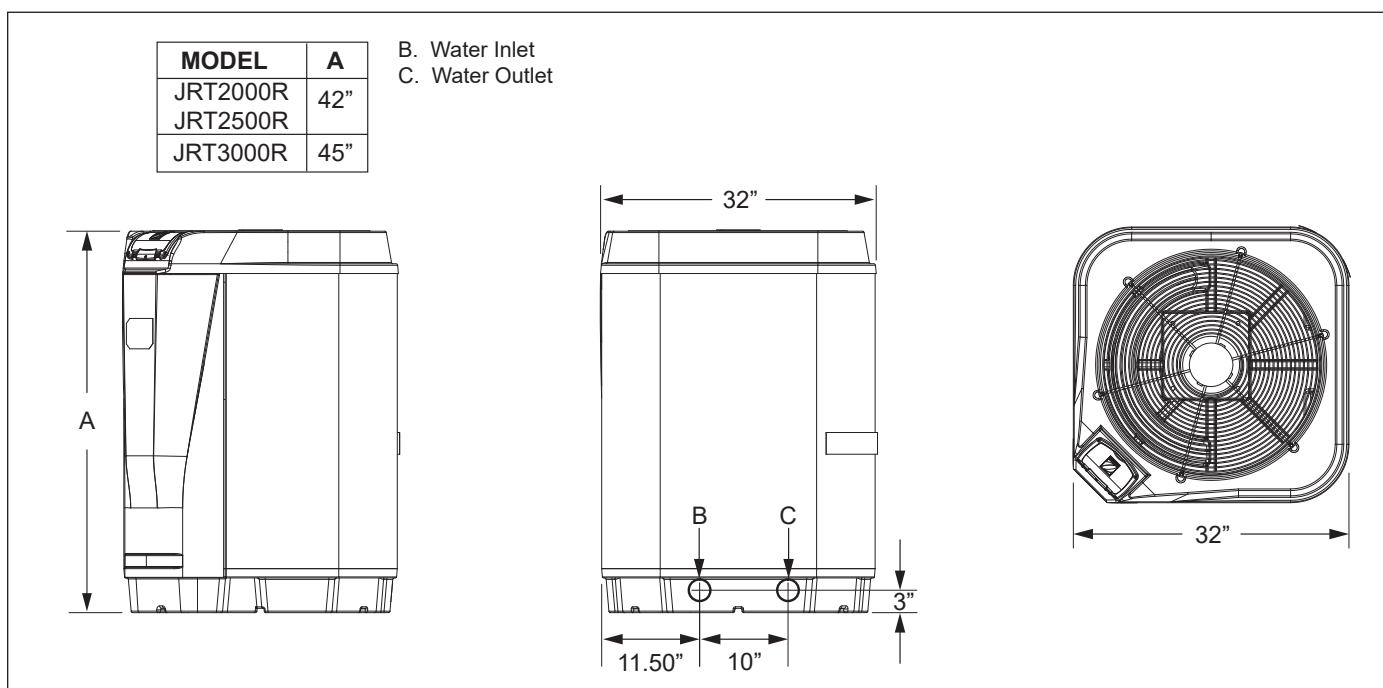
Figure 1. Jandy JRT Heat Pumps Dimensions
