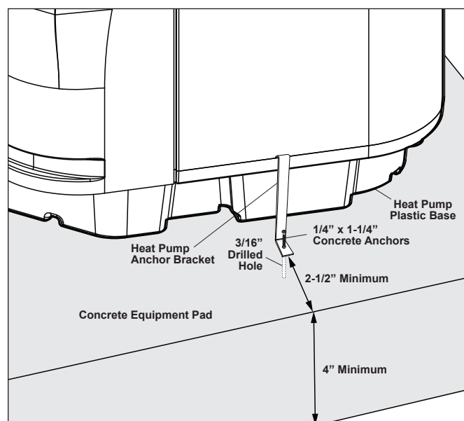
Figure 3. Anchor Clamp Installation
