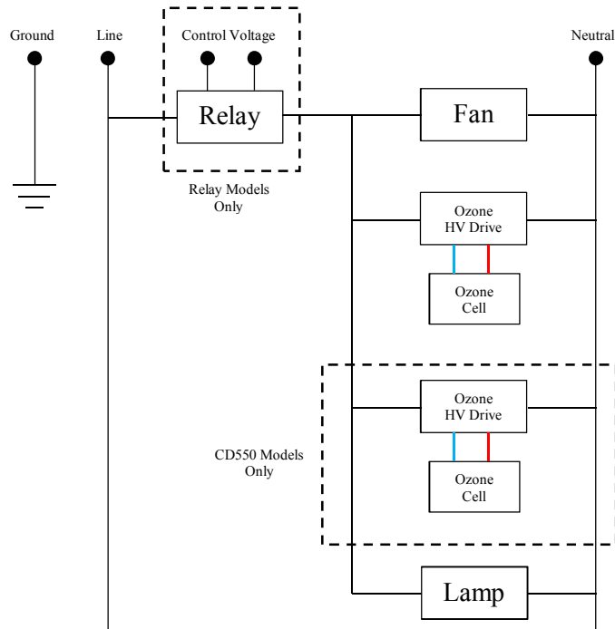
Fig 8: Wiring Schematic
