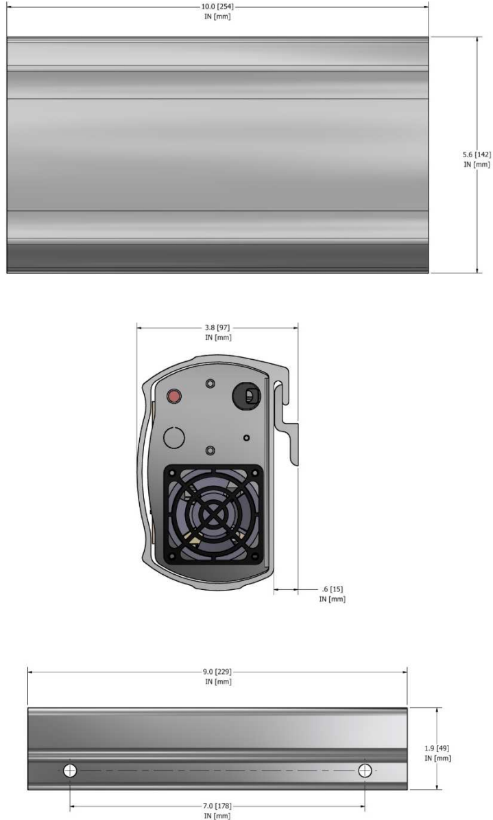
Fig 6: Overall Dimensions
