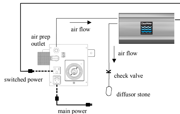
Fig 3: Diffusion Method Schematic
